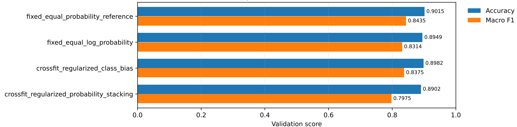
CPU screening | same cohort, cross-fitted meta methods
