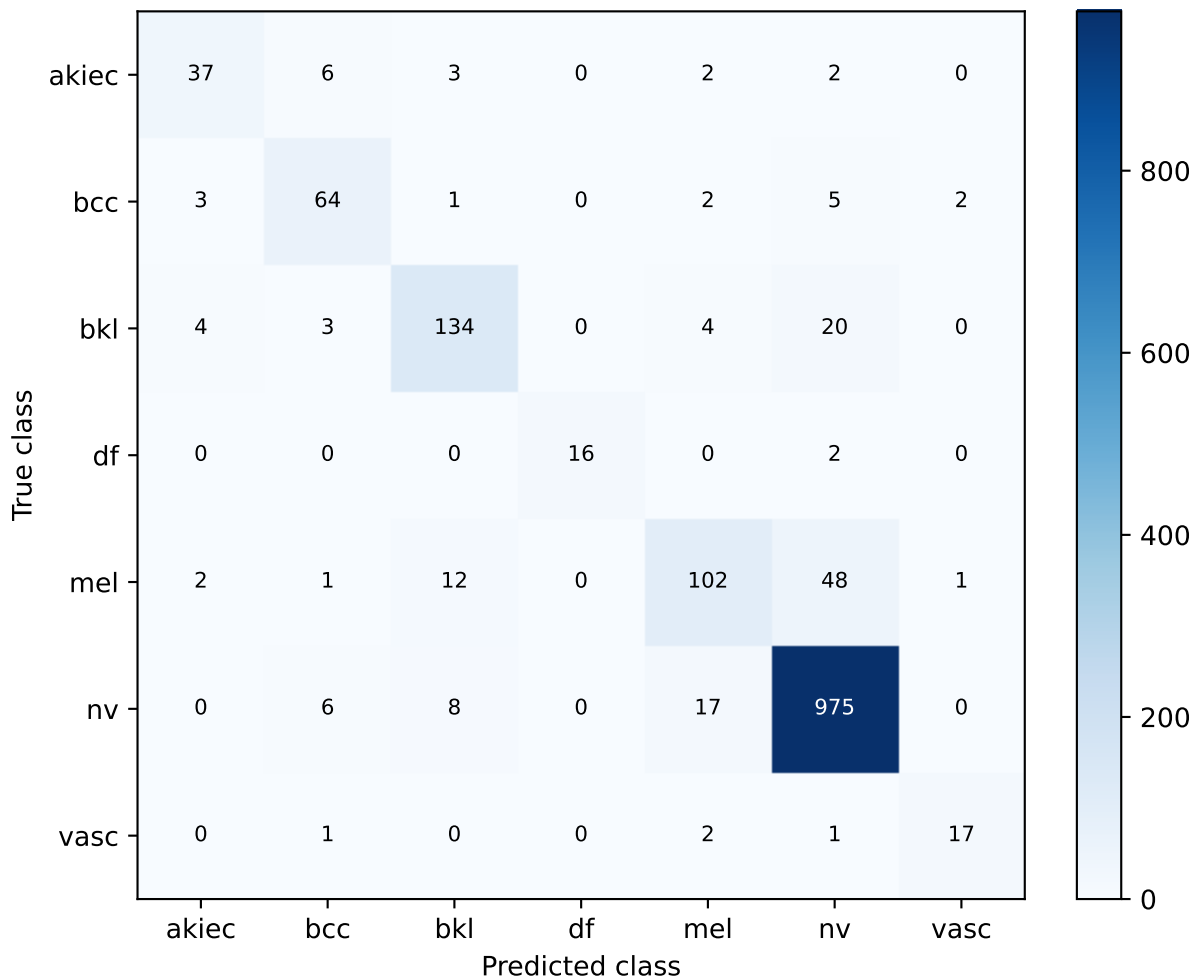
fixed_equal_log_probability | post-test development CPU screening Confusion matrix
