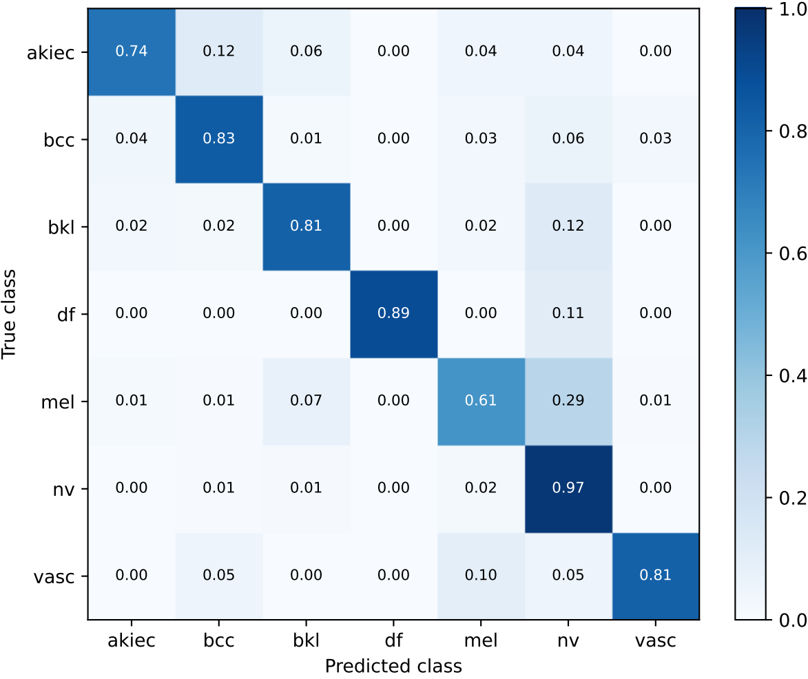
fixed_equal_log_probability | post-test development CPU screening Row-normalized confusion matrix
