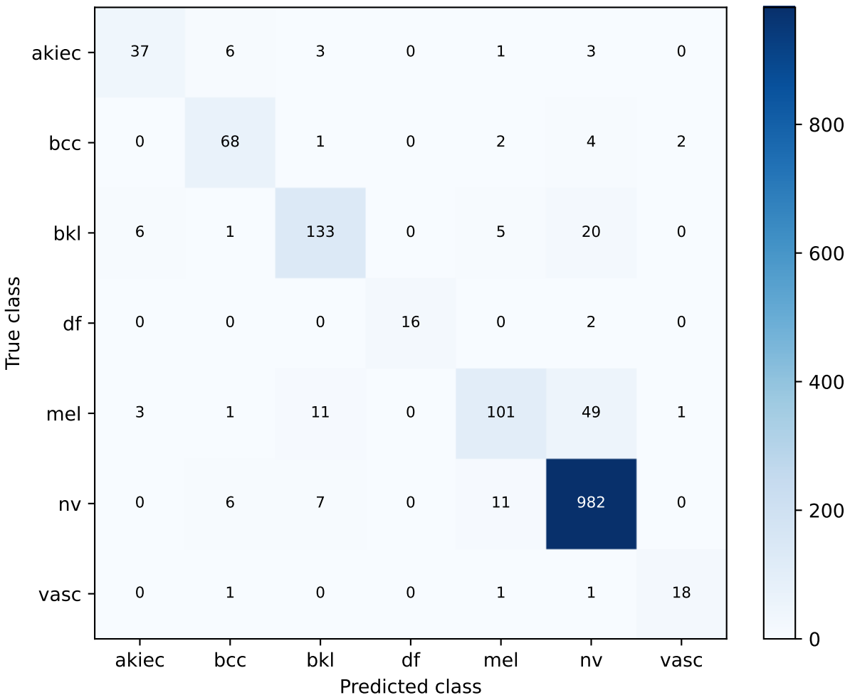
fixed_equal_probability_reference | post-test development CPU screening Confusion matrix
