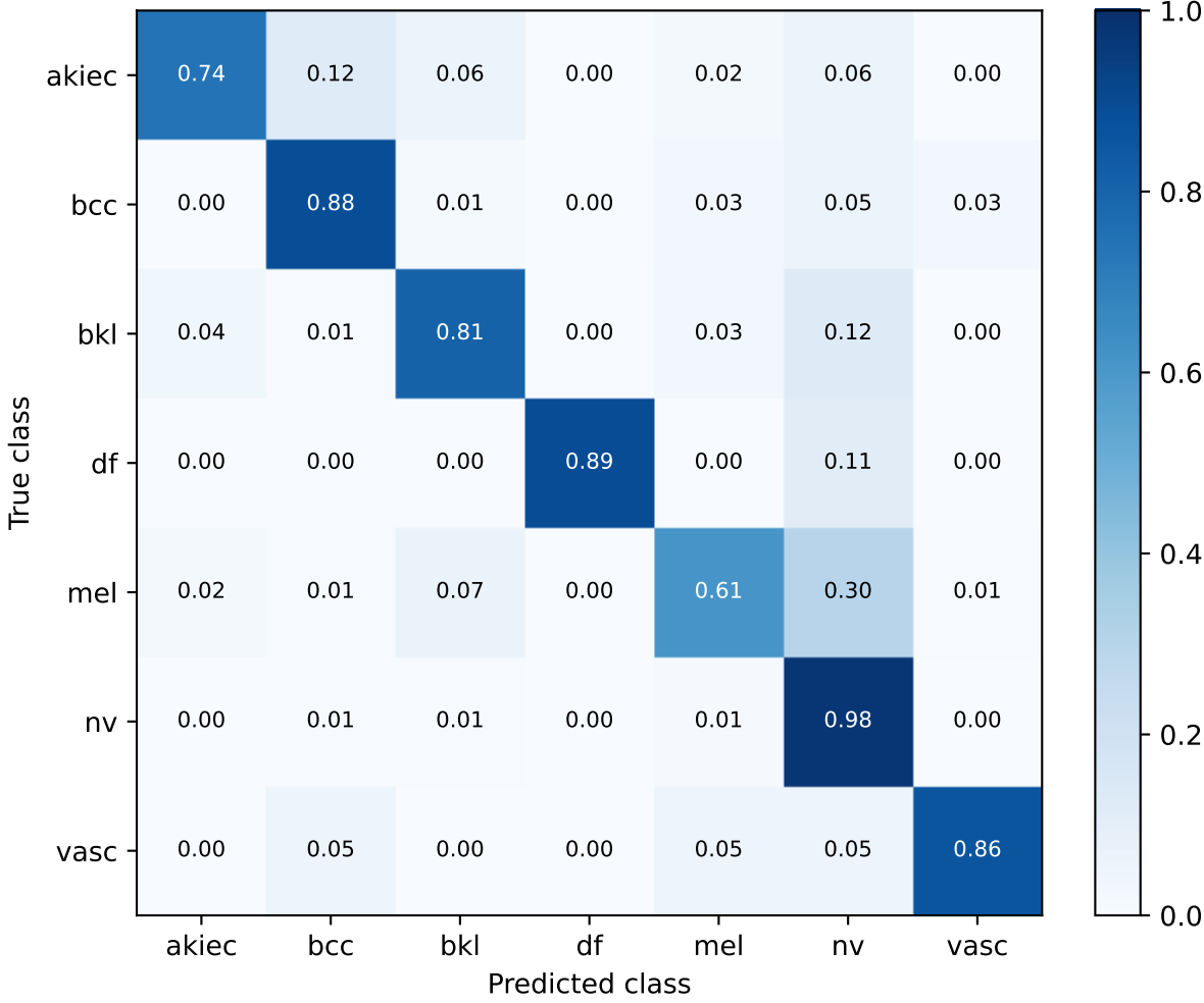
fixed_equal_probability_reference | post-test development CPU screening Row-normalized confusion matrix
