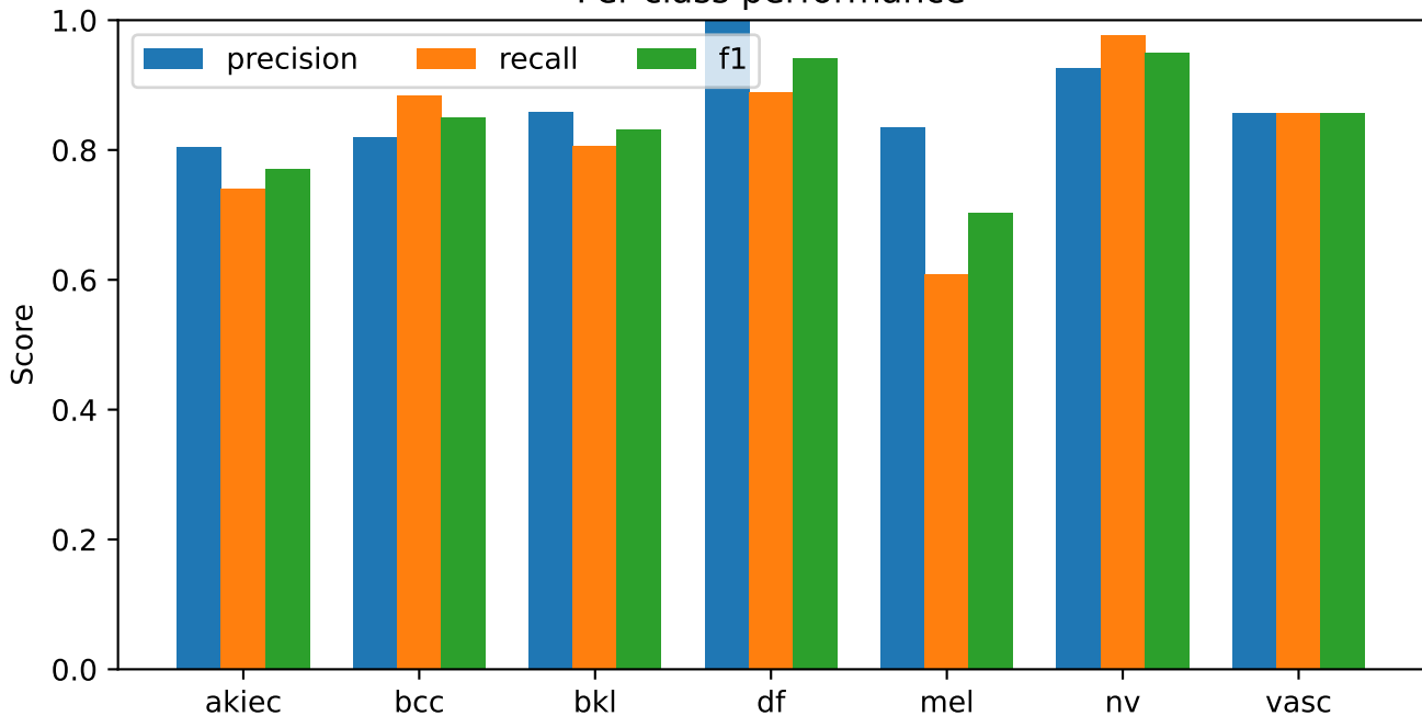
fixed_equal_probability_reference | post-test development CPU screening Per-class performance
