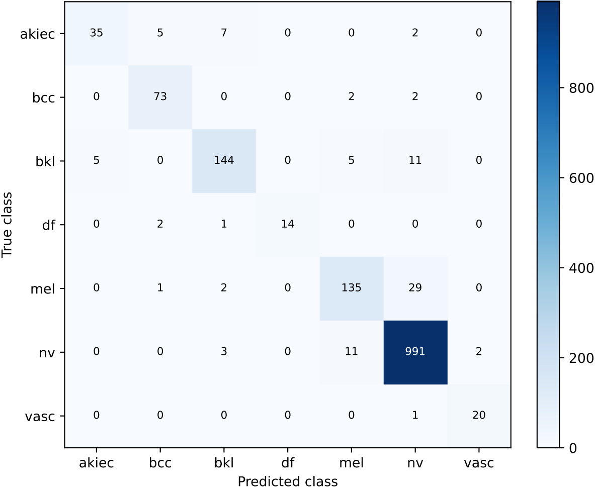
S82 fixed equal-six with Tiny and Tiny CBAM | exploratory validation Confusion matrix
