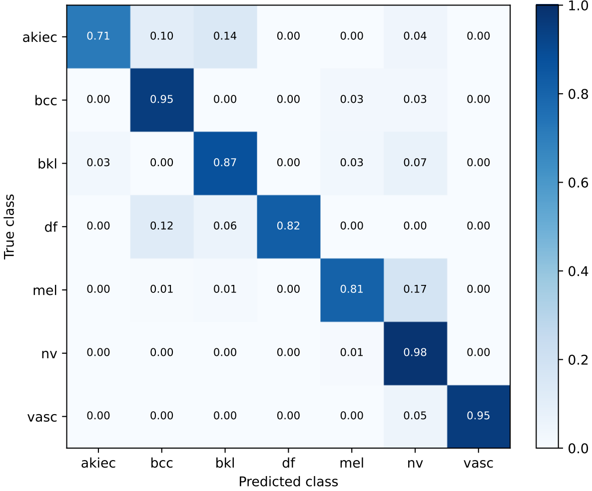
S82 fixed equal-six with Tiny and Tiny CBAM | exploratory validation Row-normalized confusion matrix
