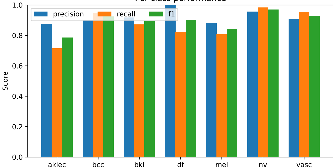
S82 fixed equal-six with Tiny and Tiny CBAM | exploratory validation Per-class performance
