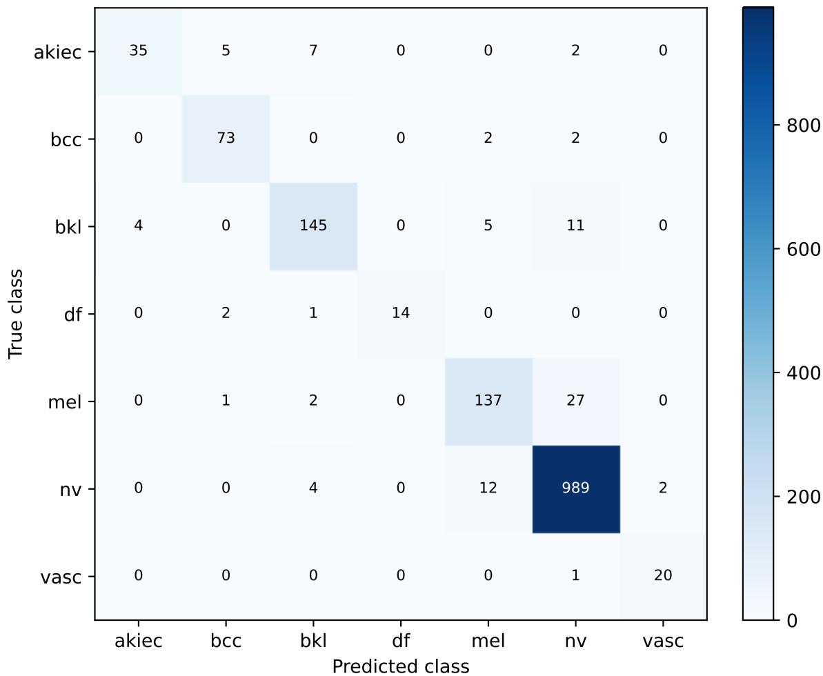
S83 equal-six with macro-F1-selected CBAM | exploratory validation Confusion matrix
