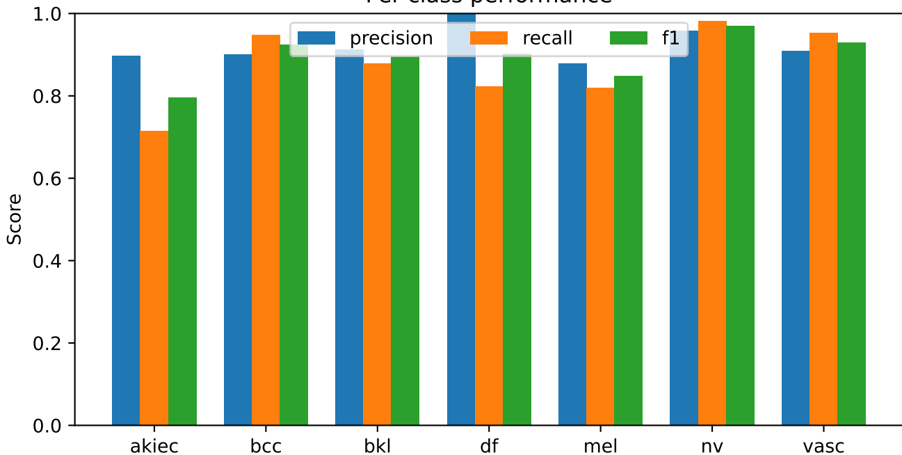
S83 equal-six with macro-F1-selected CBAM | exploratory validation Per-class performance
