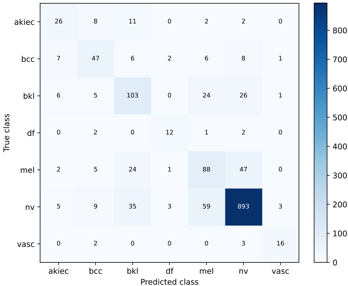
S56 frozen feature probe candidate_v2_22k | exploratory validation Confusion matrix
