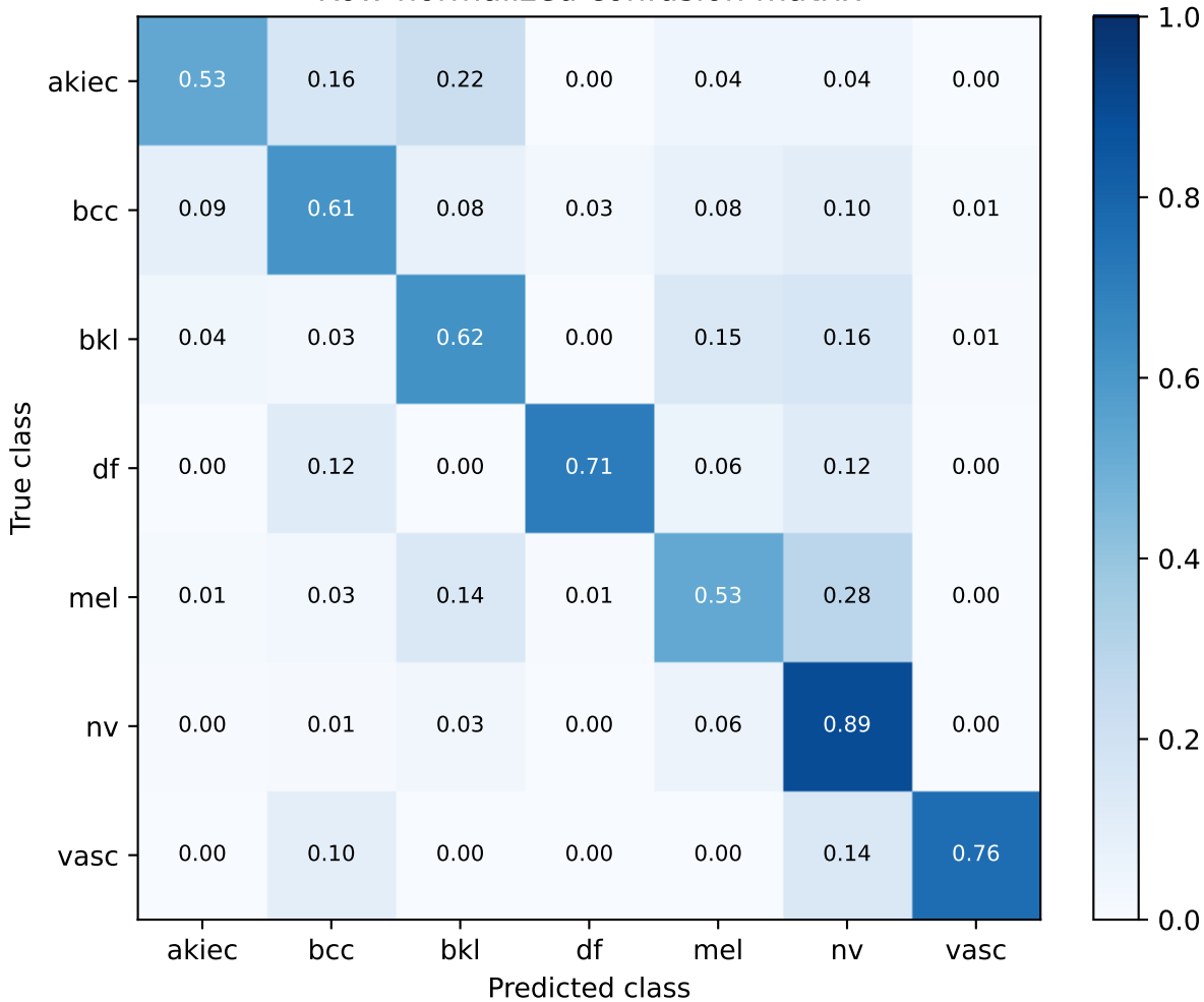
S56 frozen feature probe candidate_v2_22k | exploratory validation Row-normalized confusion matrix
