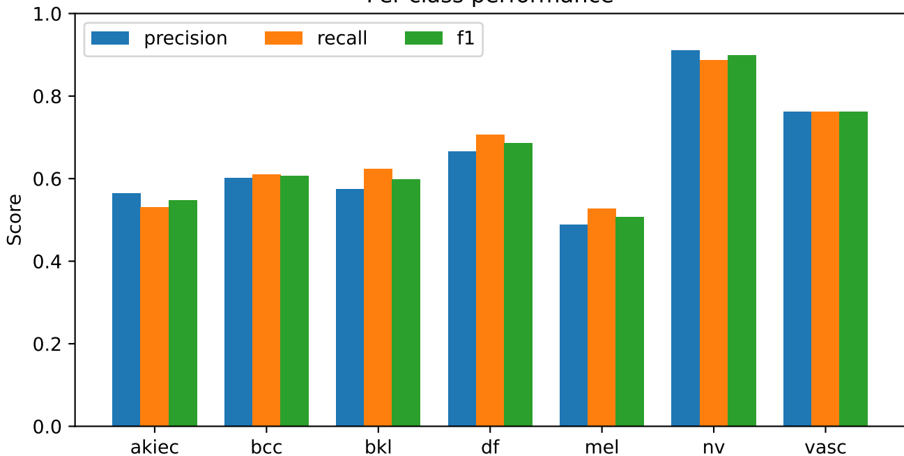
S56 frozen feature probe candidate_v2_22k | exploratory validation Per-class performance
