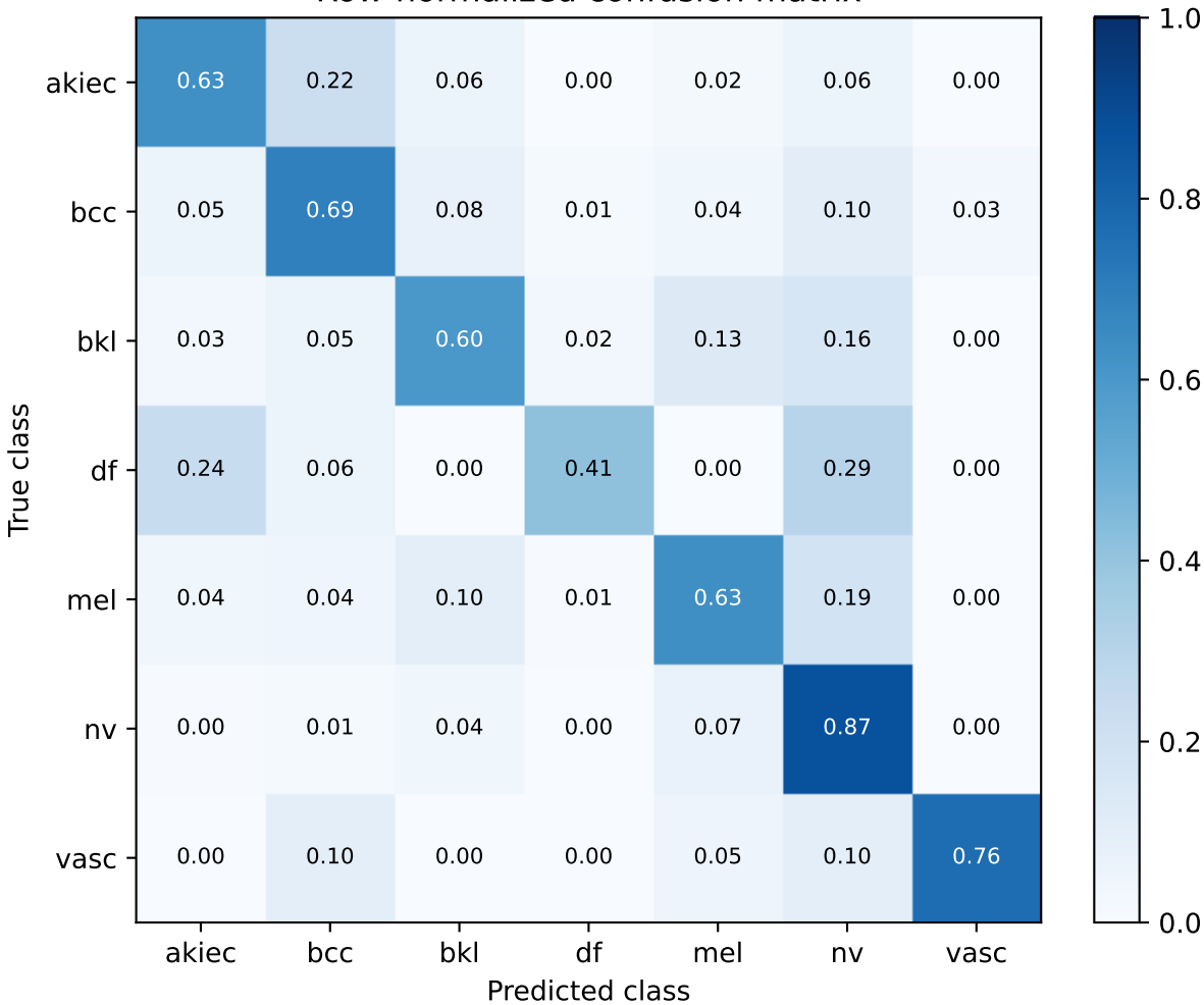
S56 frozen feature probe control_1k | exploratory validation Row-normalized confusion matrix
