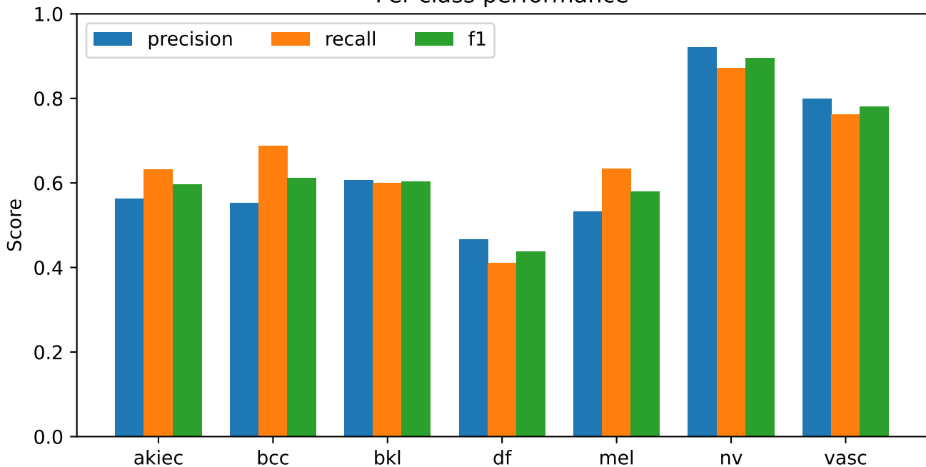
S56 frozen feature probe control_1k | exploratory validation Per-class performance
