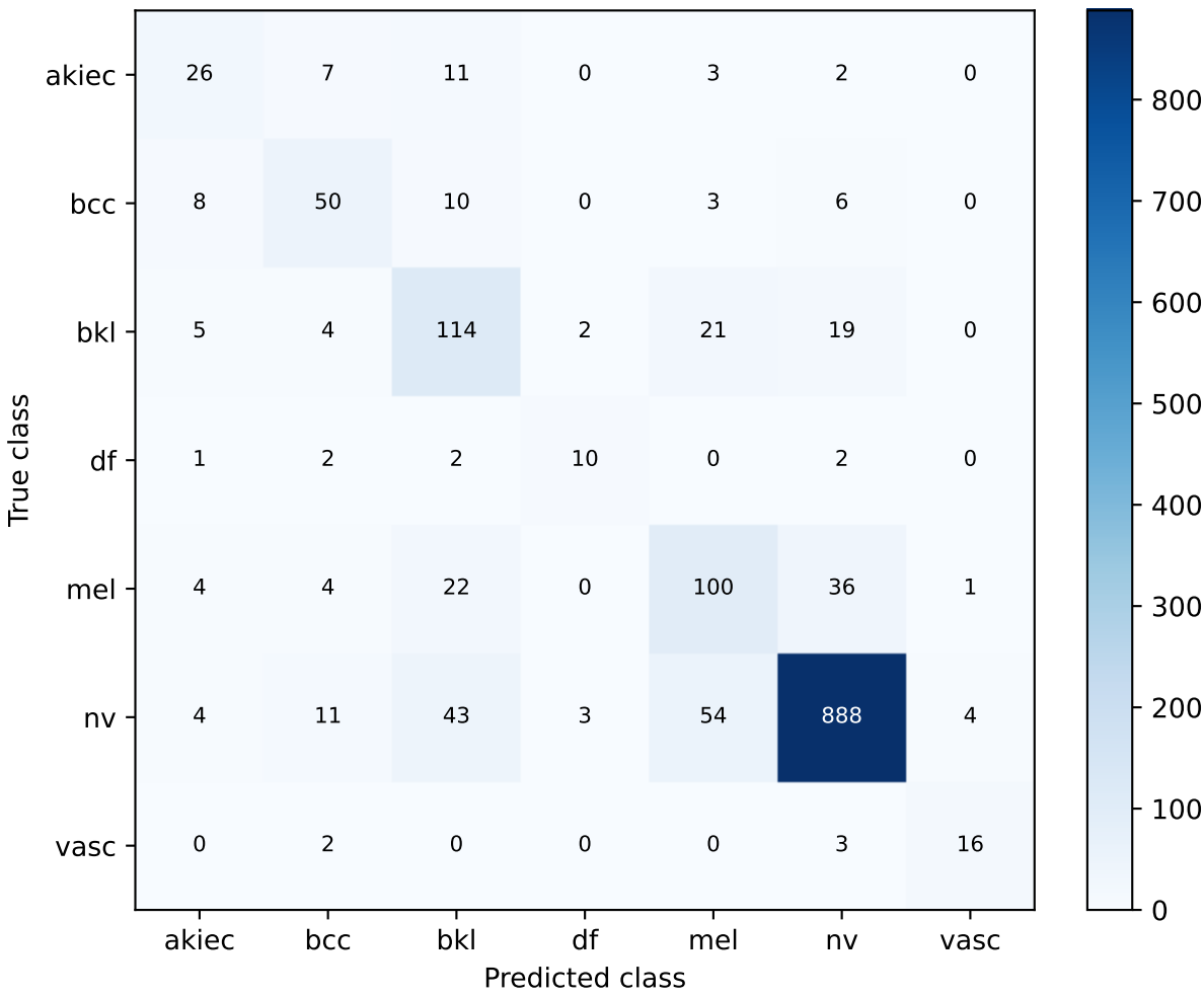
S58 frozen feature probe candidate_supervised22k | exploratory validation Confusion matrix
