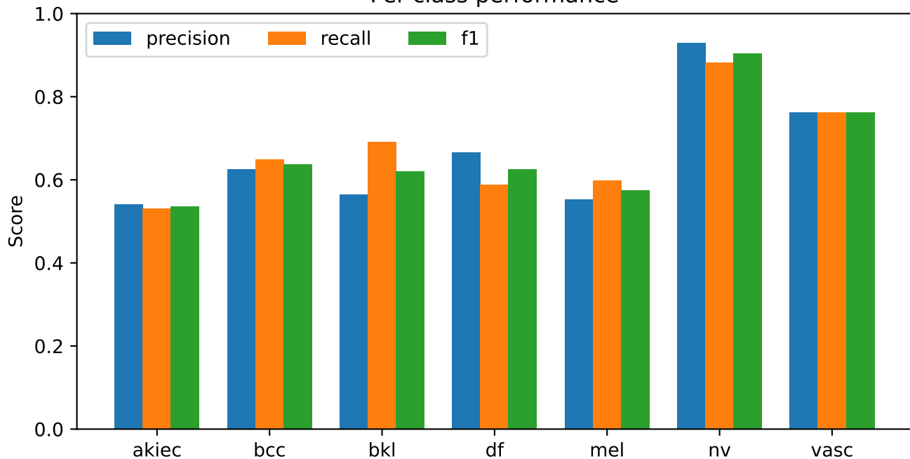
S58 frozen feature probe candidate_supervised22k | exploratory validation Per-class performance
