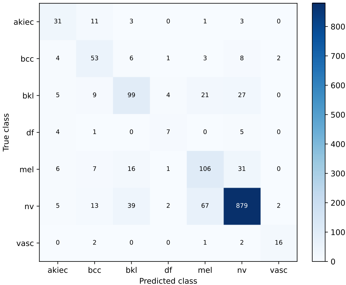
S58 frozen feature probe control_1k | exploratory validation Confusion matrix
