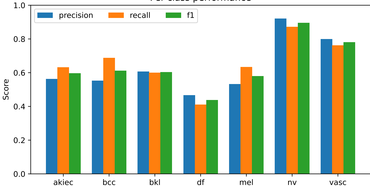
S58 frozen feature probe control_1k | exploratory validation Per-class performance
