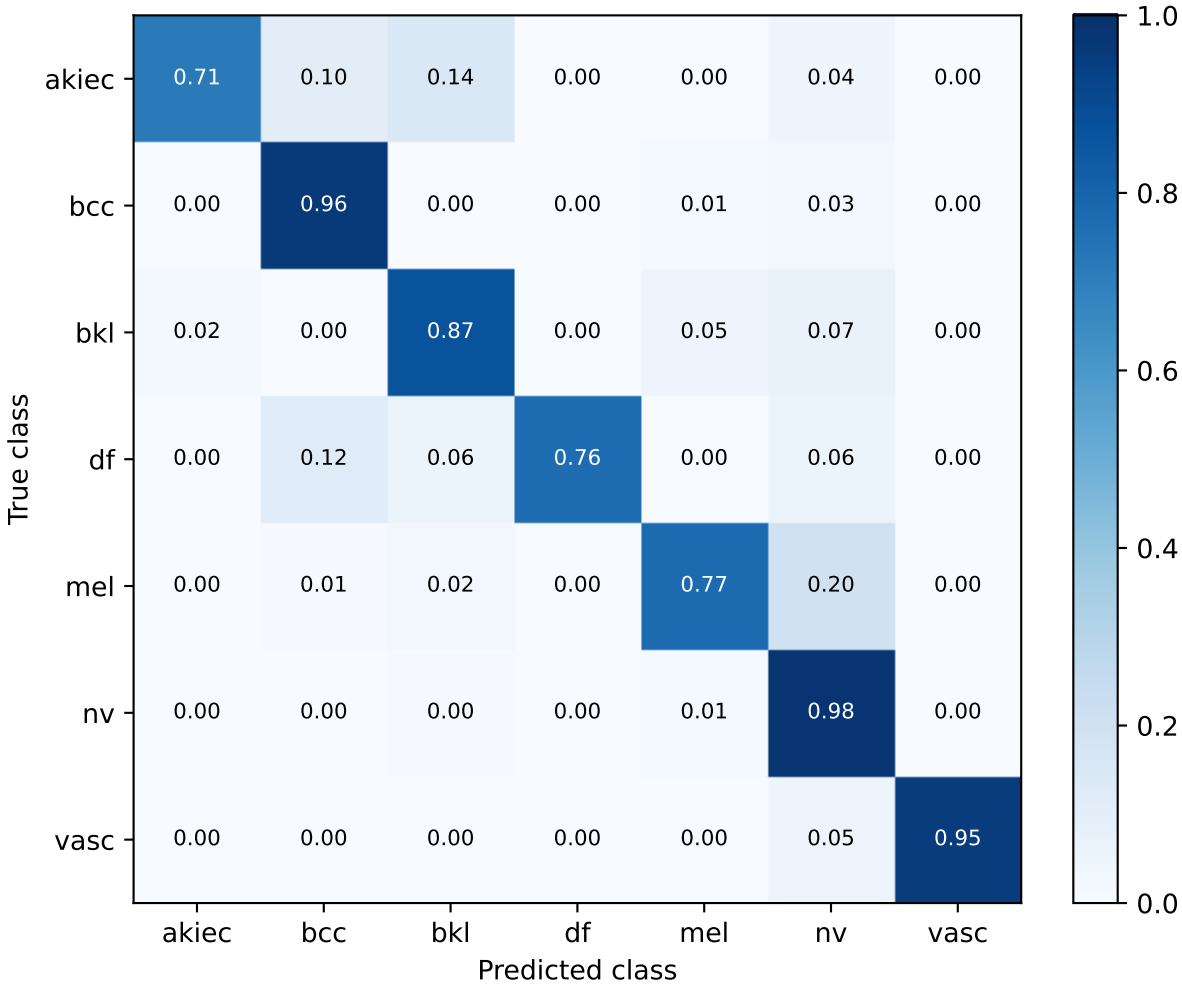
S60 fixed S59 fusion | exploratory validation Row-normalized confusion matrix
