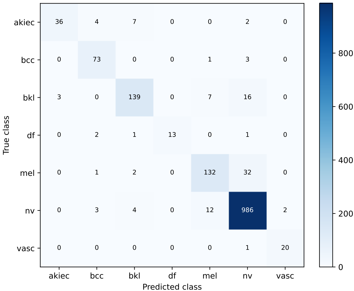
S61 fixed S59 fusion | exploratory validation Confusion matrix
