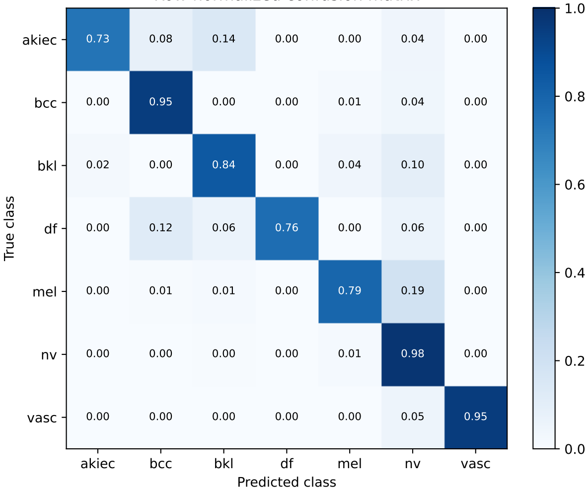
S61 fixed S59 fusion | exploratory validation Row-normalized confusion matrix
