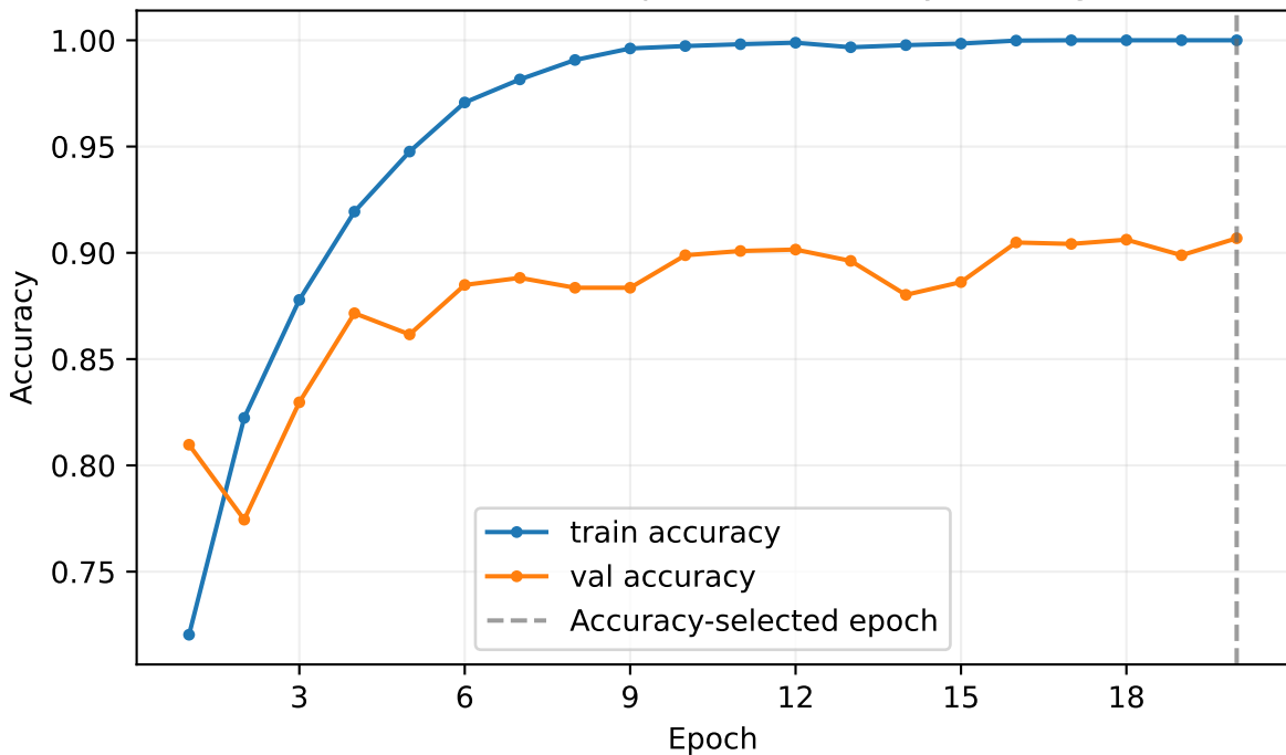
S59 ConvNeXt supervised22k Tiny training
