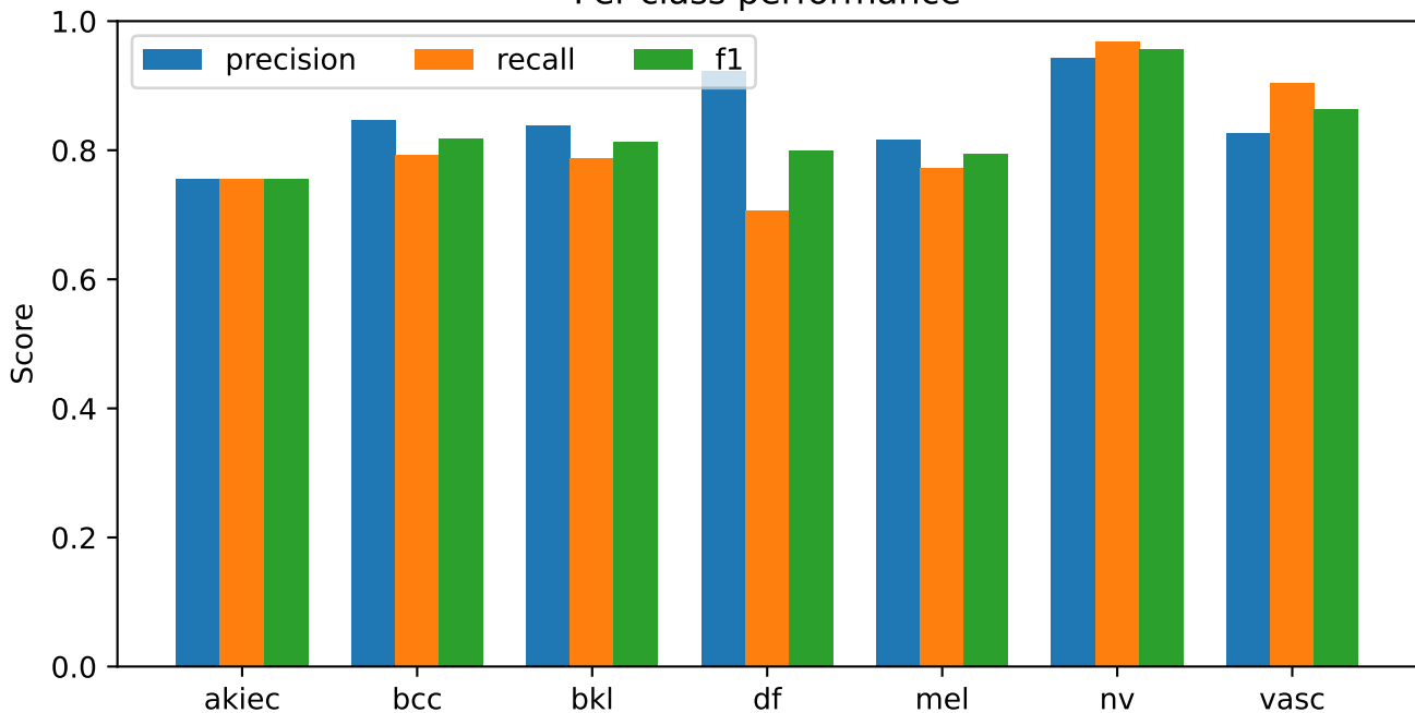
S59 ConvNeXt supervised22k Tiny | exploratory validation Per-class performance
