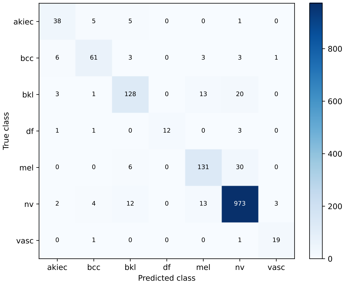
S59 ConvNeXt supervised22k Tiny | exploratory validation_macro_f1 Confusion matrix
