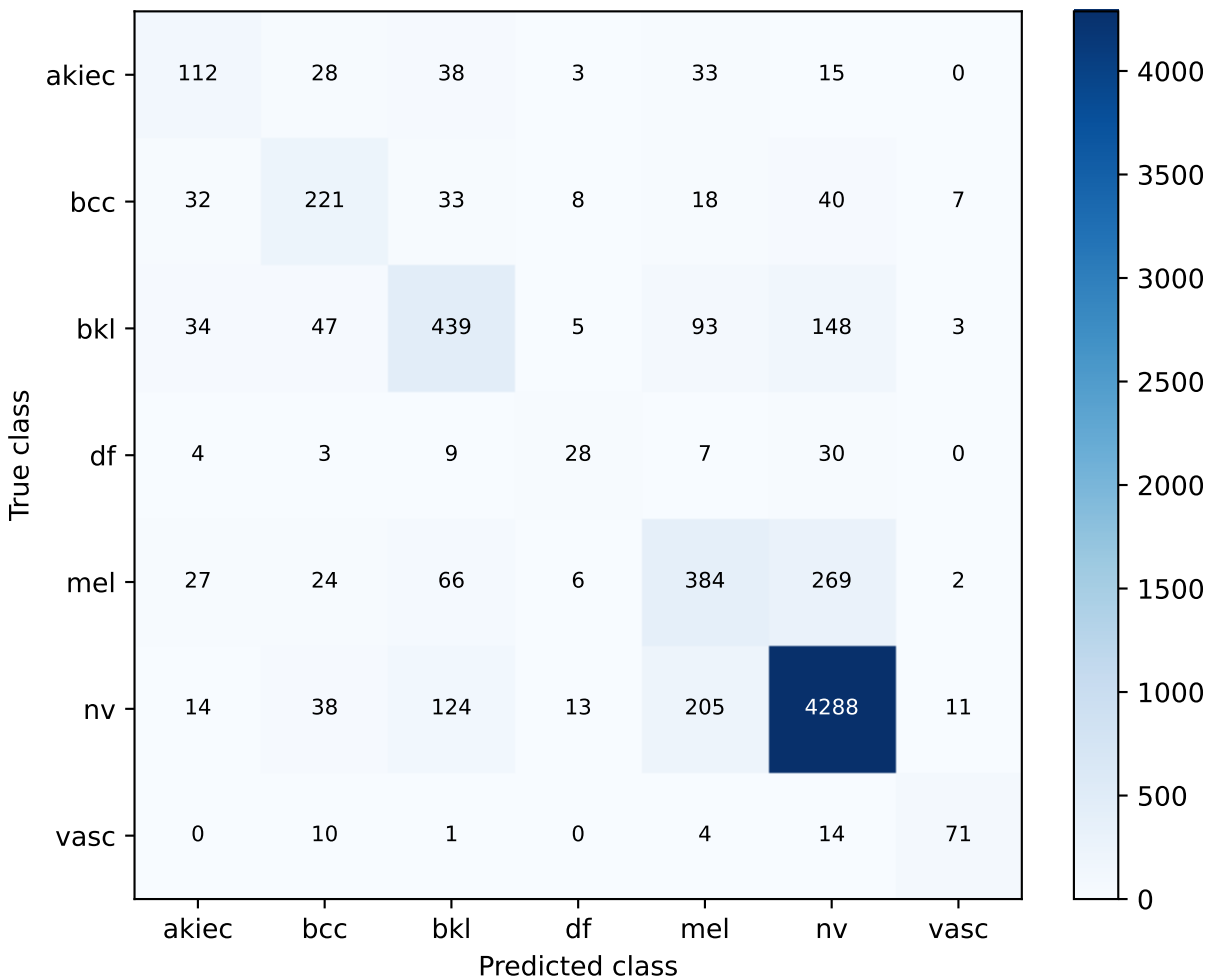
S74 image_weighted | train-only lesion-group OOF Confusion matrix
