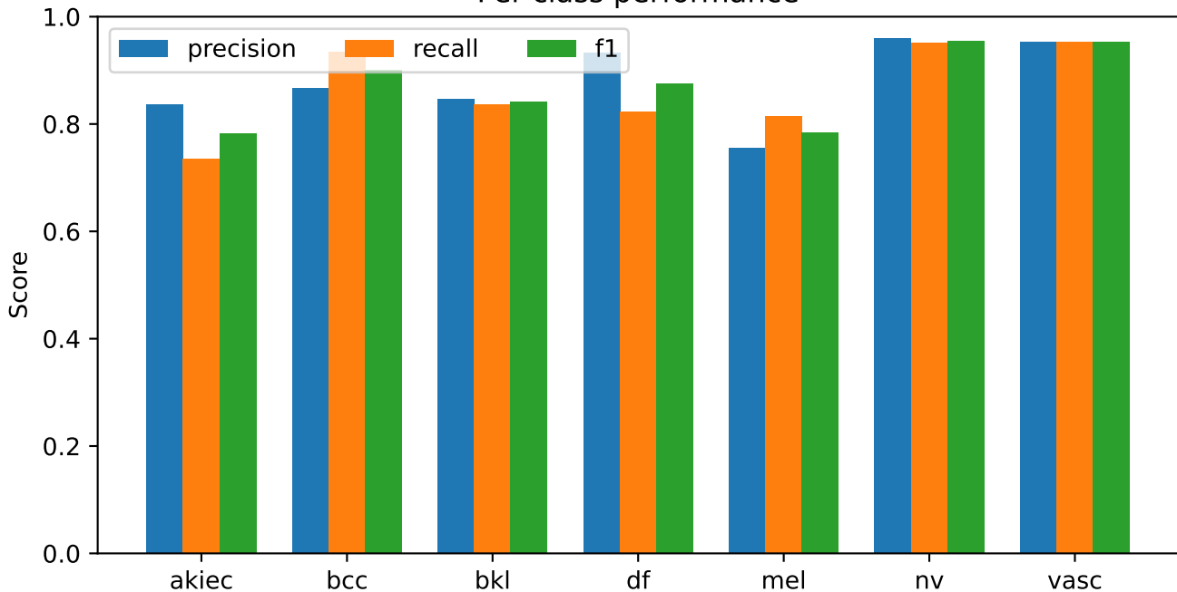
S75 averaged_tiny_cpu | exploratory validation Per-class performance
