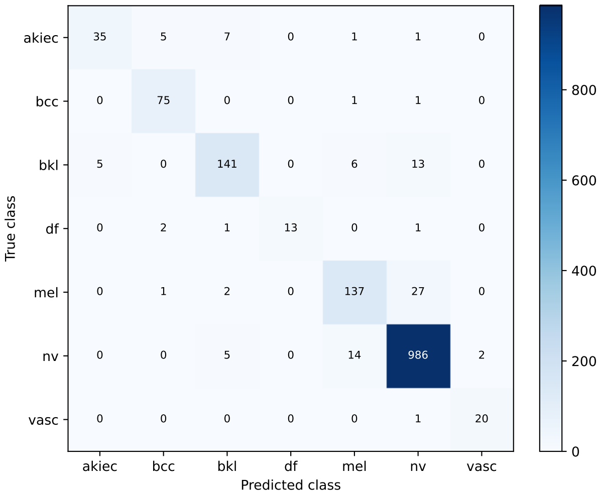
S75 equal_five_cpu_tiny_control | exploratory validation Confusion matrix
