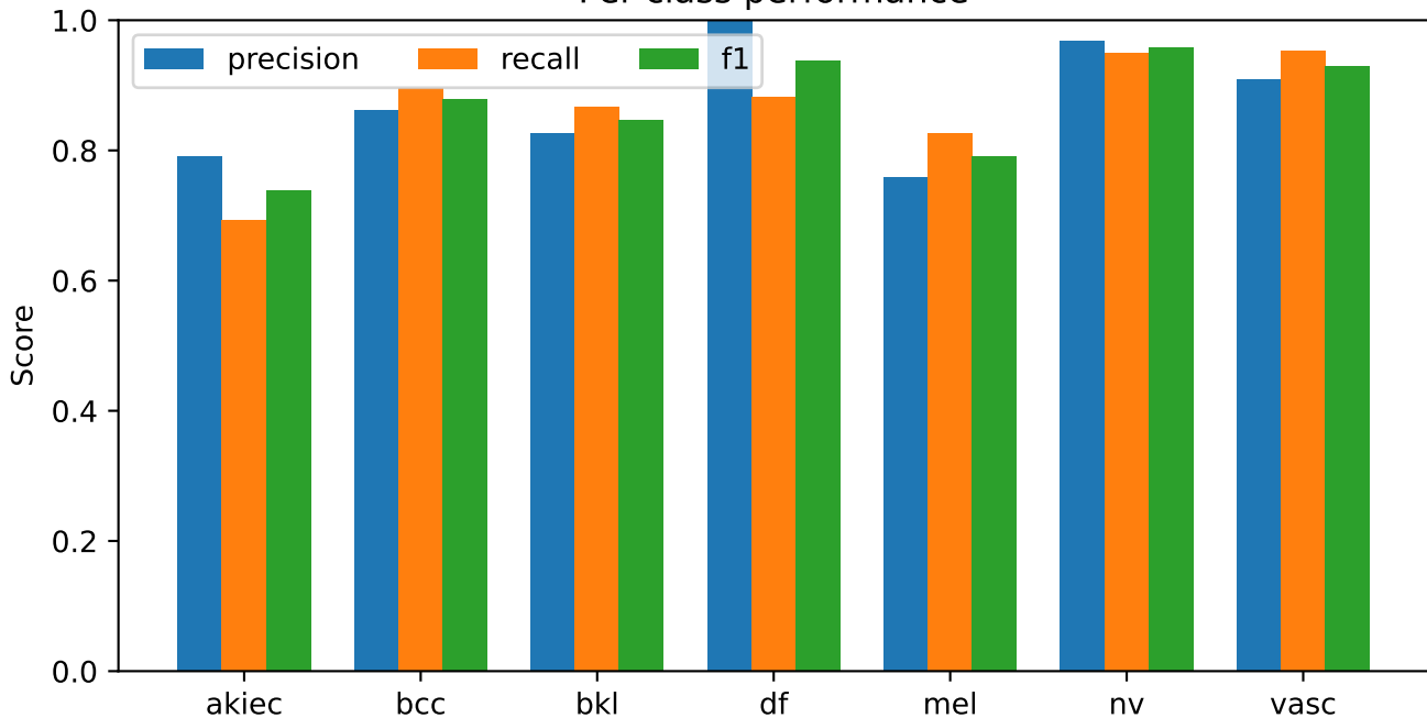
S75 original_tiny_cpu_control | exploratory validation Per-class performance
