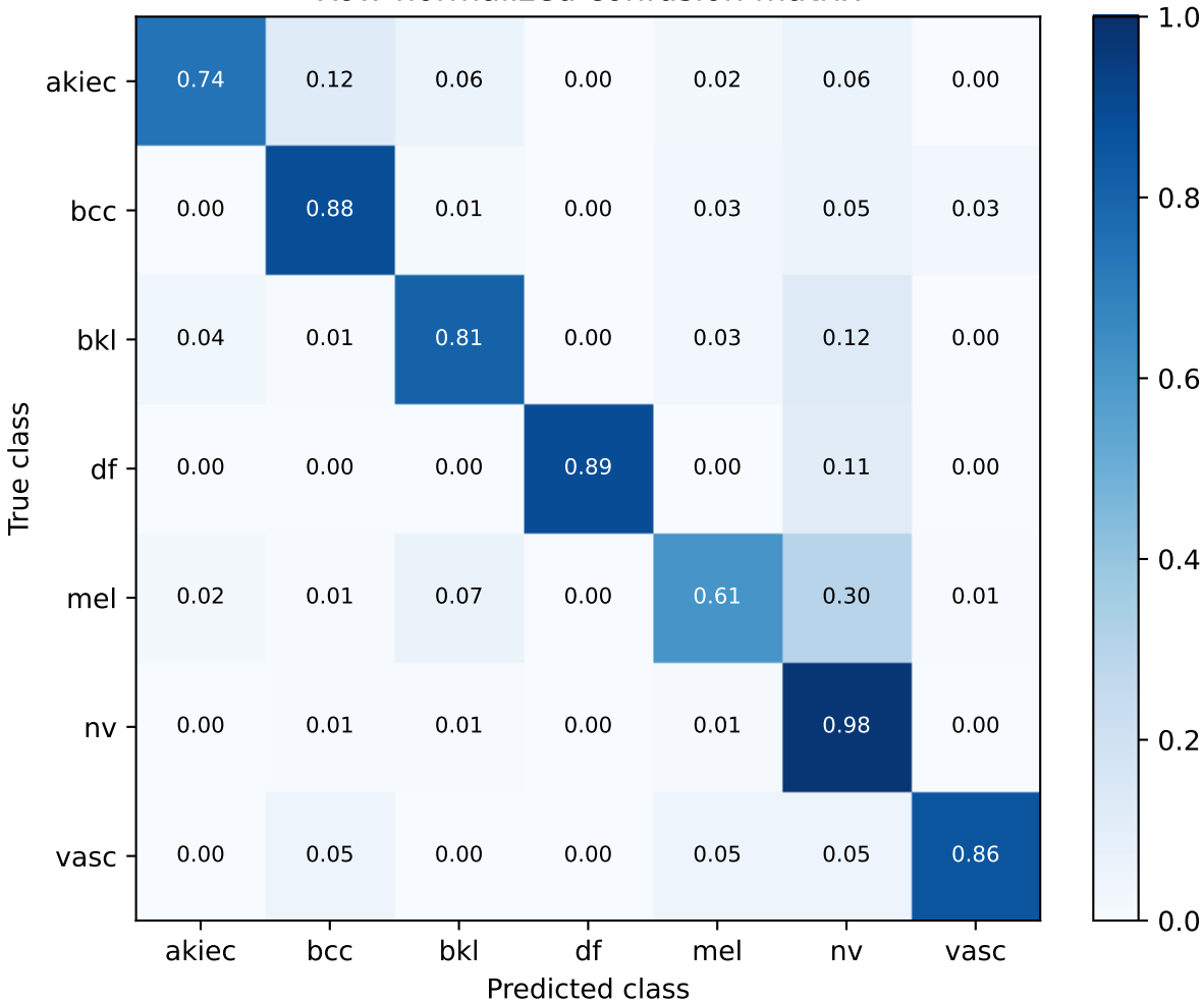
Frozen equal ensemble | strict lesion-disjoint validation Row-normalized confusion matrix
