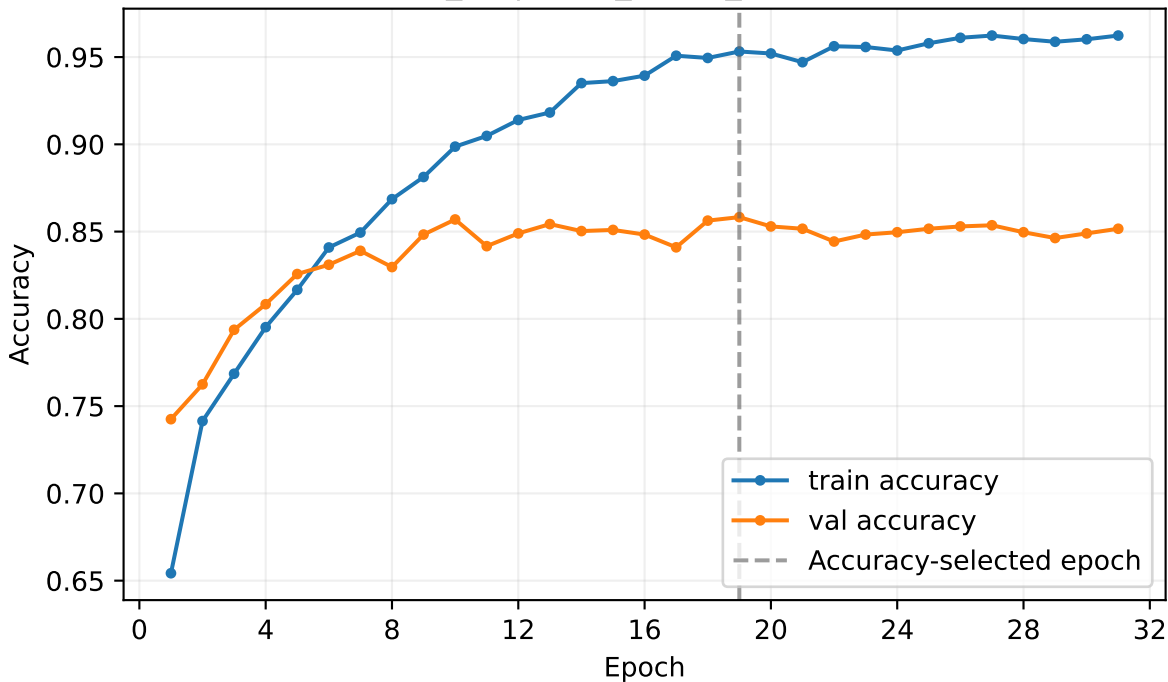
efficientnet_b0 | strict_lesion_disjoint validation
