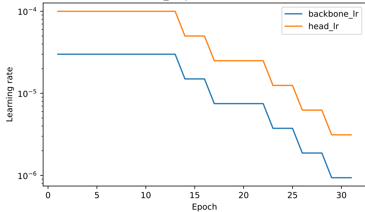
efficientnet_b0 | strict validation recipe
