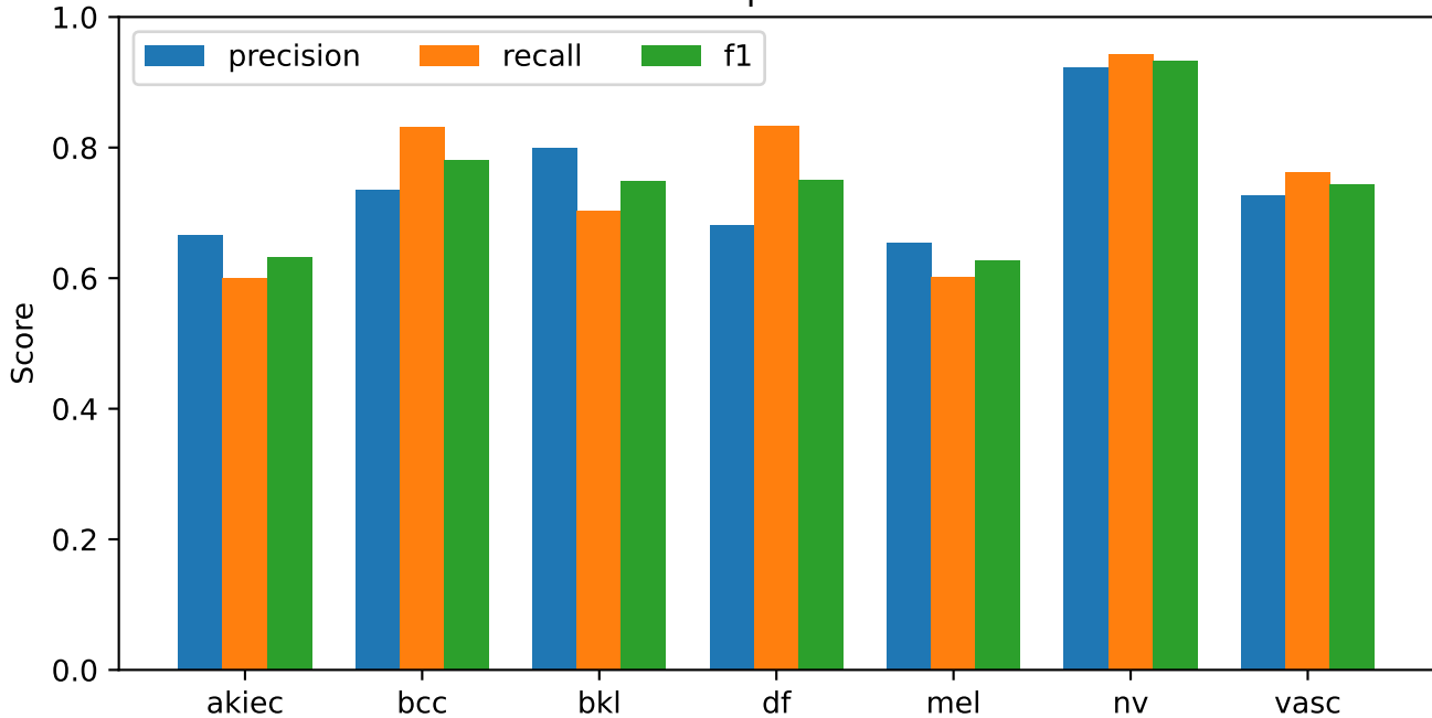
efficientnet_b0 | strict_lesion_disjoint validation Per-class performance
