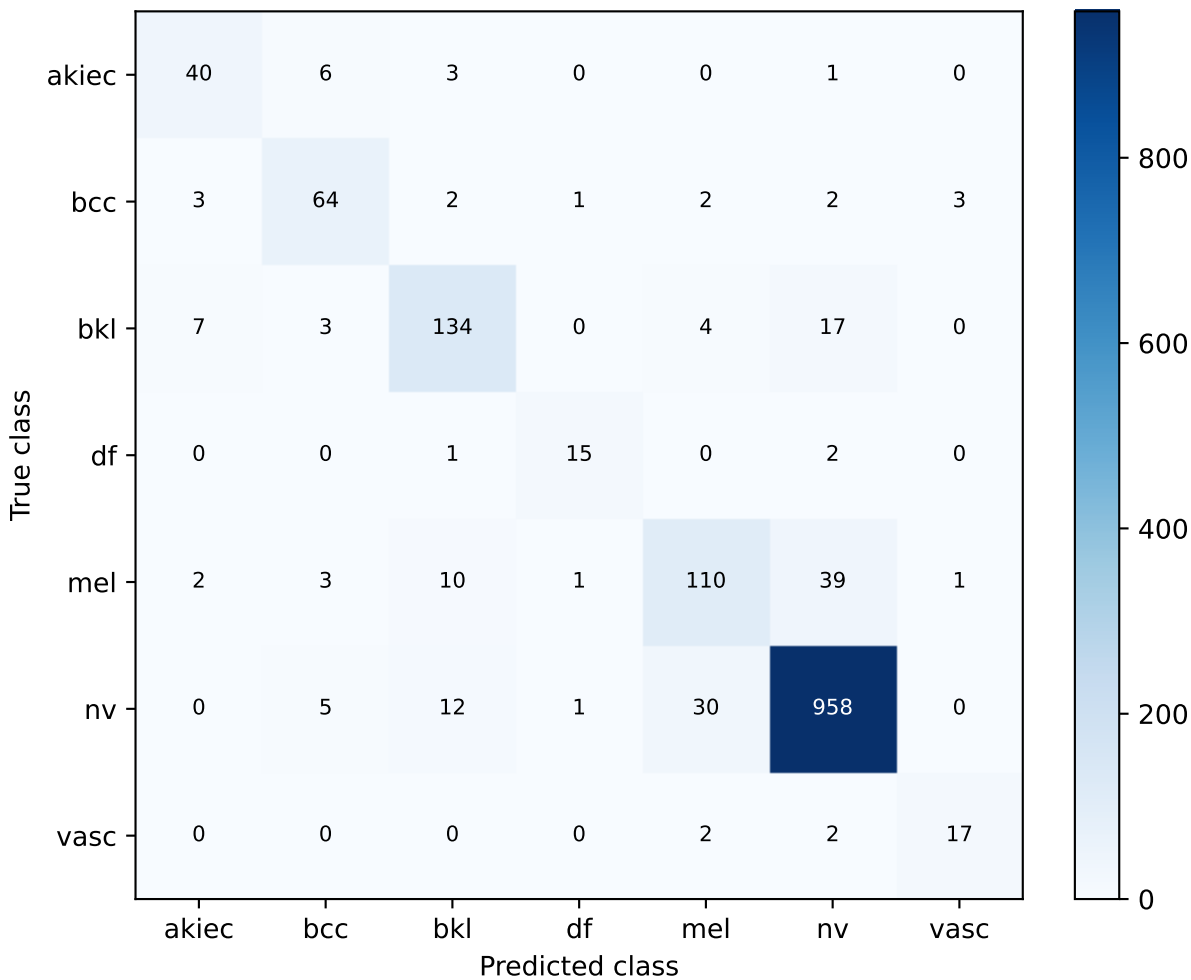
convnext_tiny | strict_lesion_disjoint validation Confusion matrix
