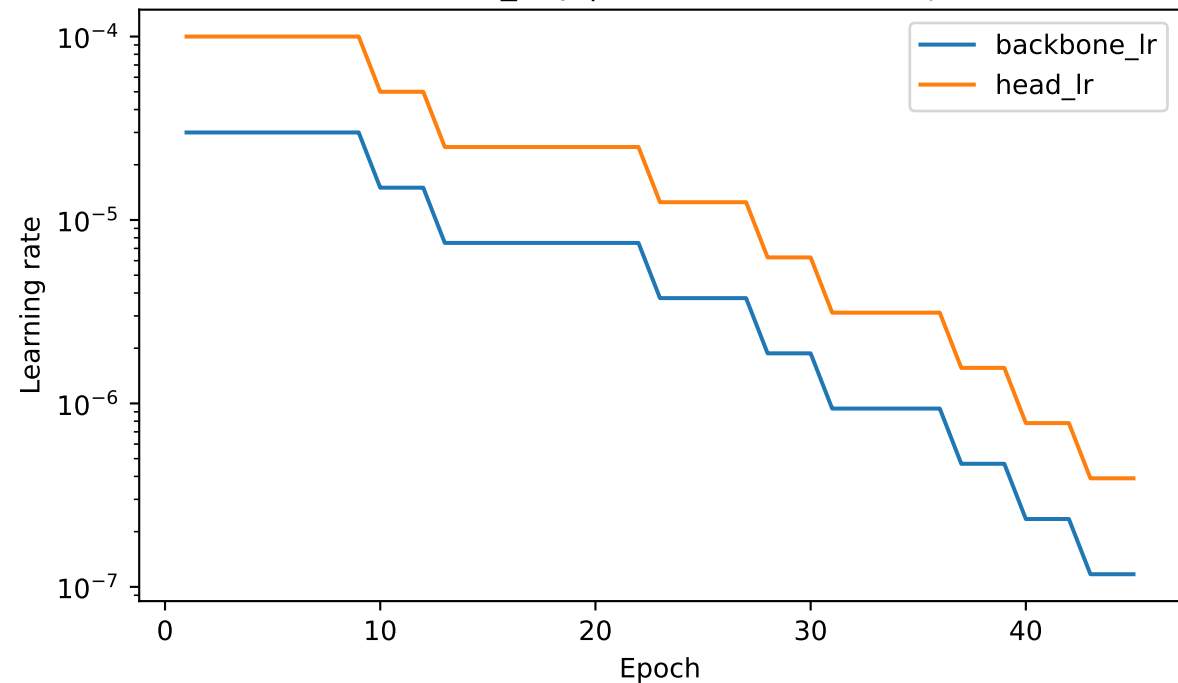
convnext_tiny | strict validation recipe
