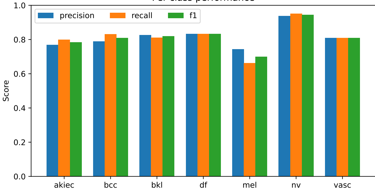
convnext_tiny | strict_lesion_disjoint validation Per-class performance
