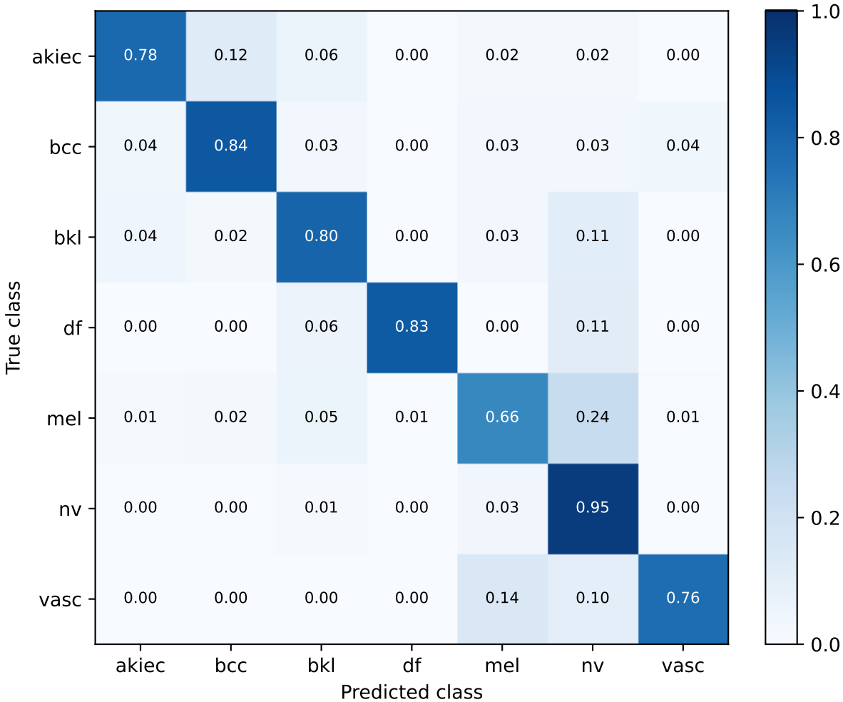
Final strict validation | latest checkpoint Row-normalized confusion matrix
