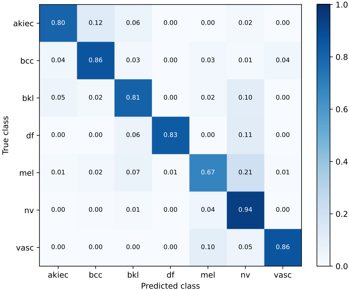
Final strict validation | macro-F1 checkpoint Row-normalized confusion matrix
