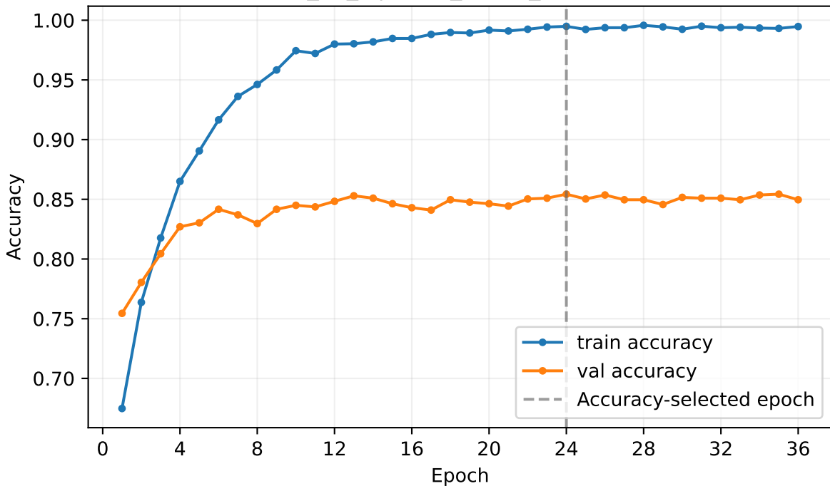
efficientnet_v2_s | strict_lesion_disjoint validation
