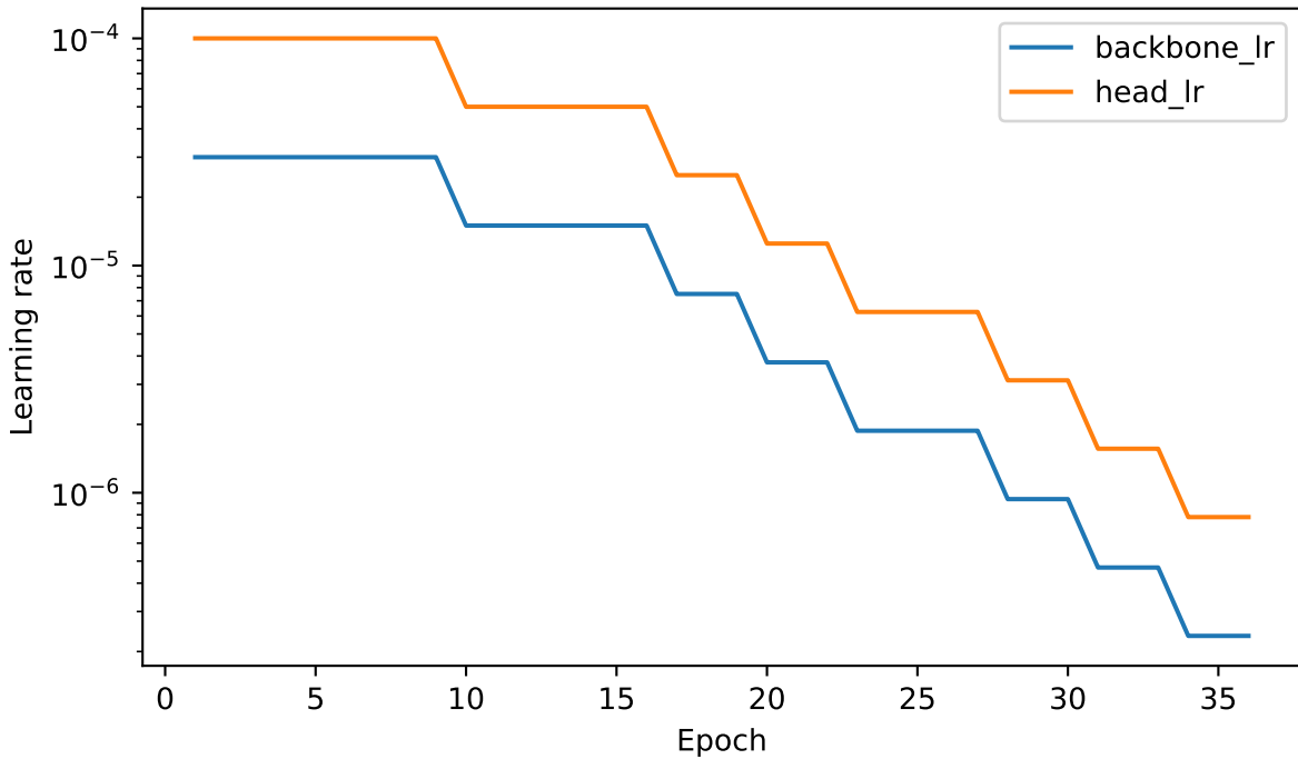
efficientnet_v2_s | strict validation recipe
