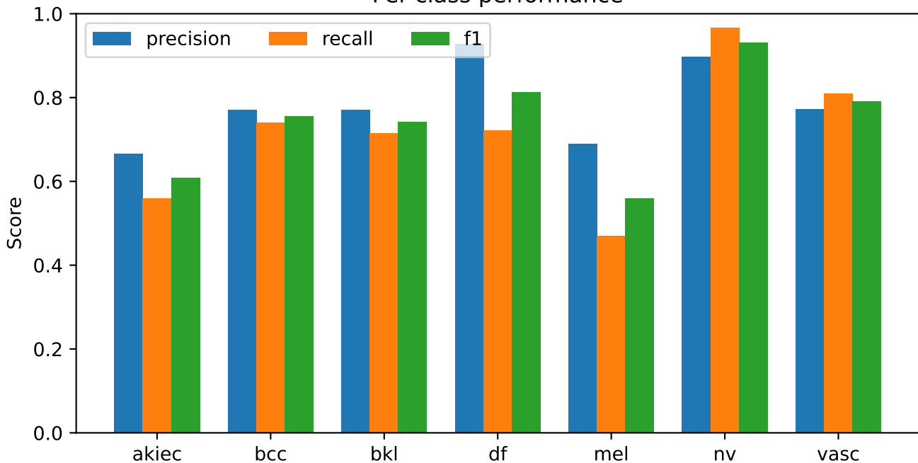
efficientnet_v2_s | strict_lesion_disjoint validation Per-class performance
