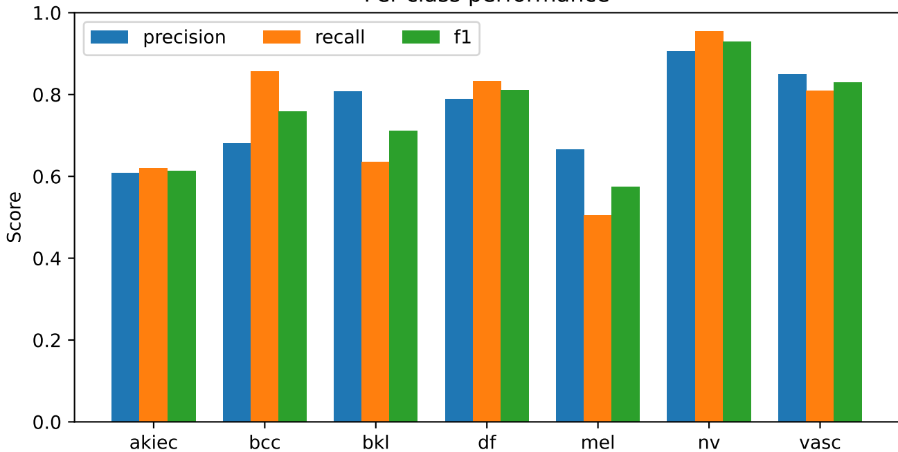
Final strict validation | macro-F1 checkpoint Per-class performance
