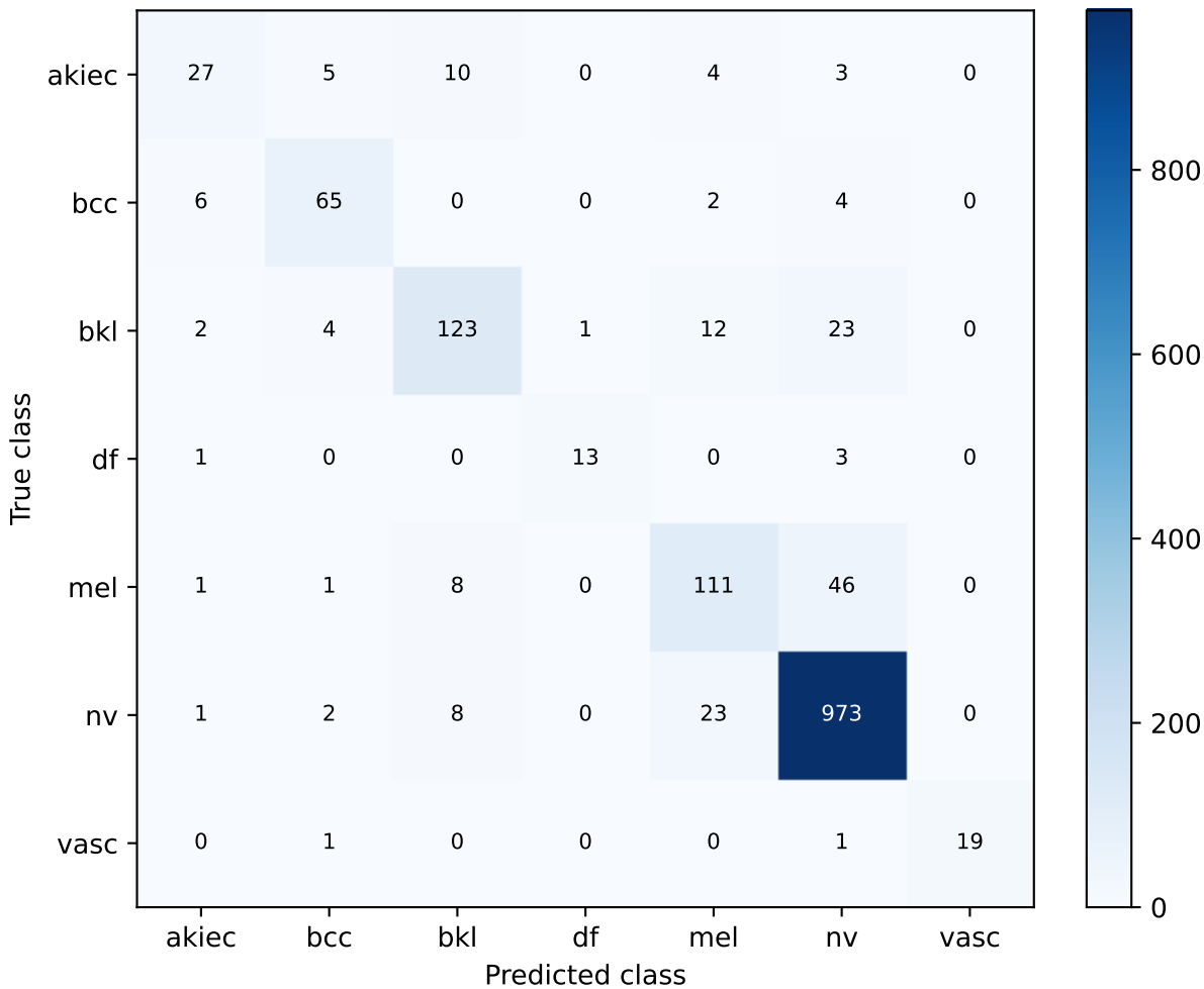
base | exploratory development Confusion matrix
