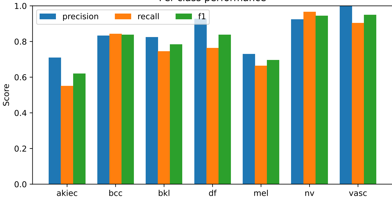
base | exploratory development Per-class performance
