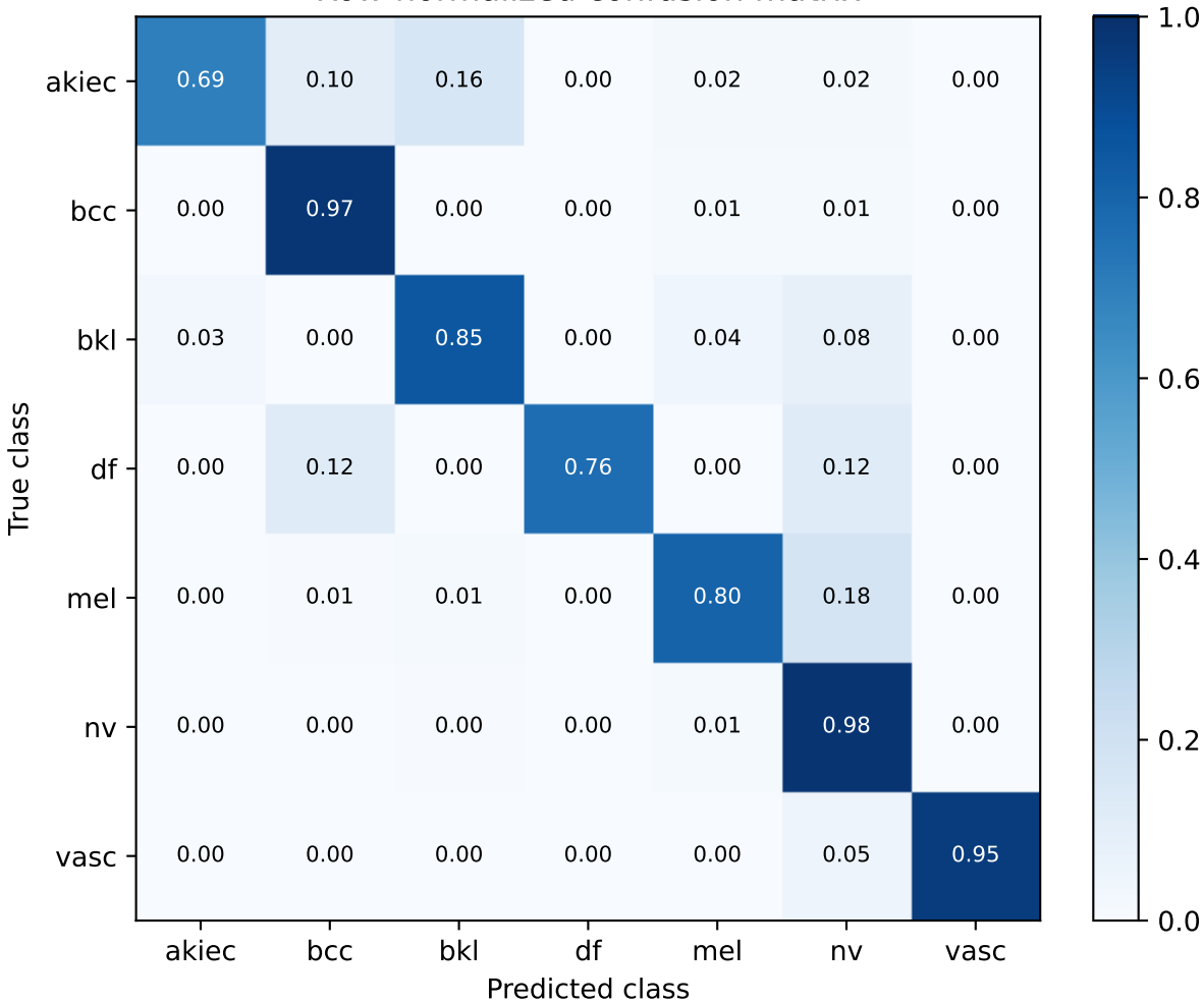
S54 fixed PanDerm fusion | exploratory validation Row-normalized confusion matrix
