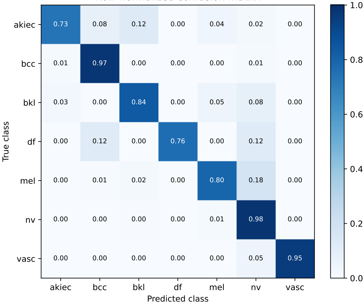
S55 fixed PanDerm fusion | exploratory validation Row-normalized confusion matrix
