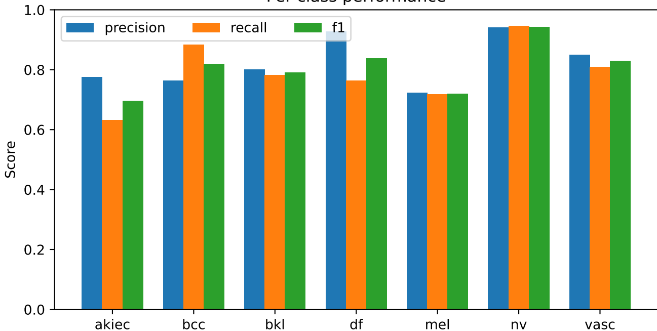
S04 fixed equal fusion | exploratory validation | no weight tuning Per-class performance
