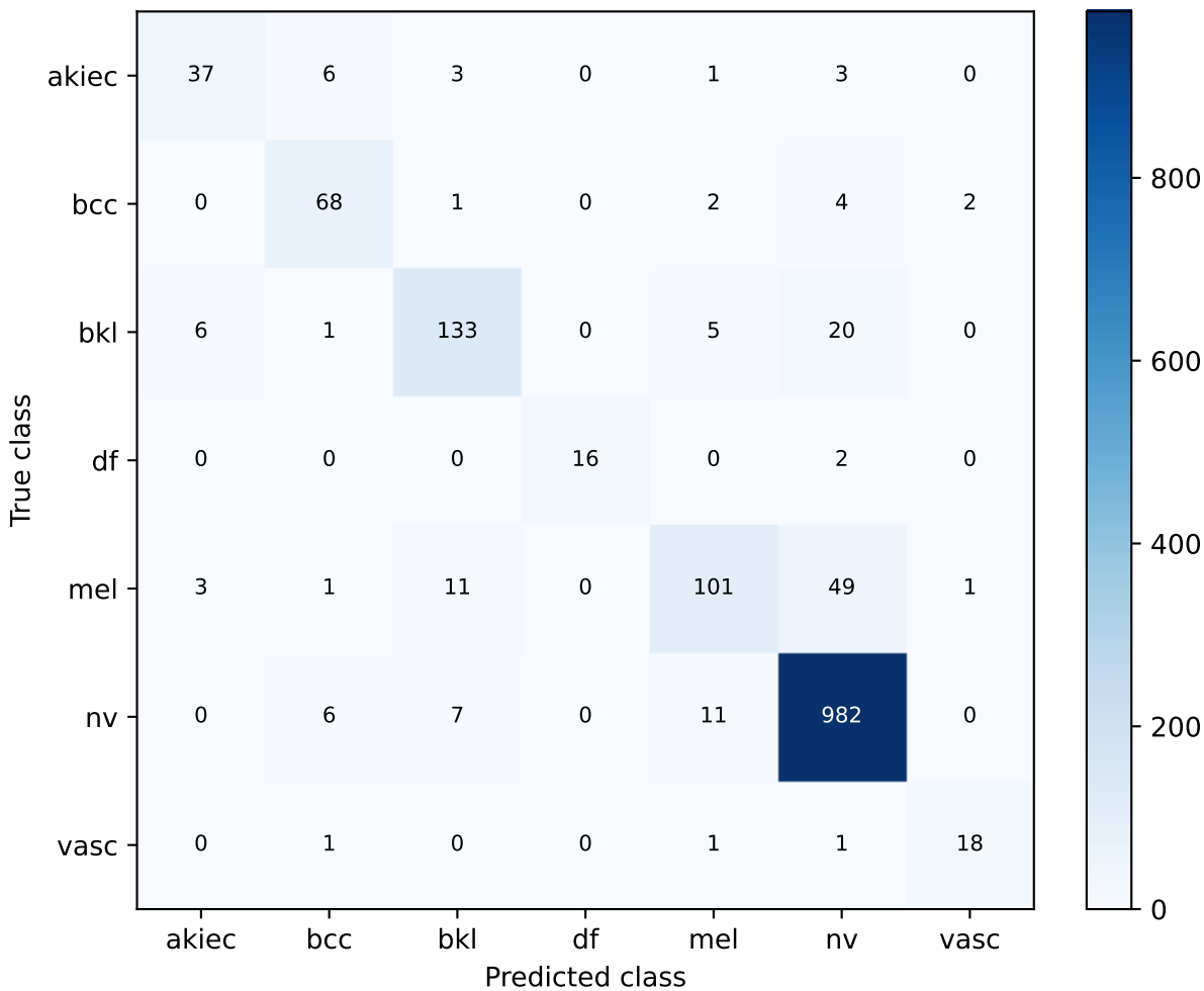
s37_convnext_control_strict_dev_seed42 | fixed B0 + candidate + V2S Confusion matrix
