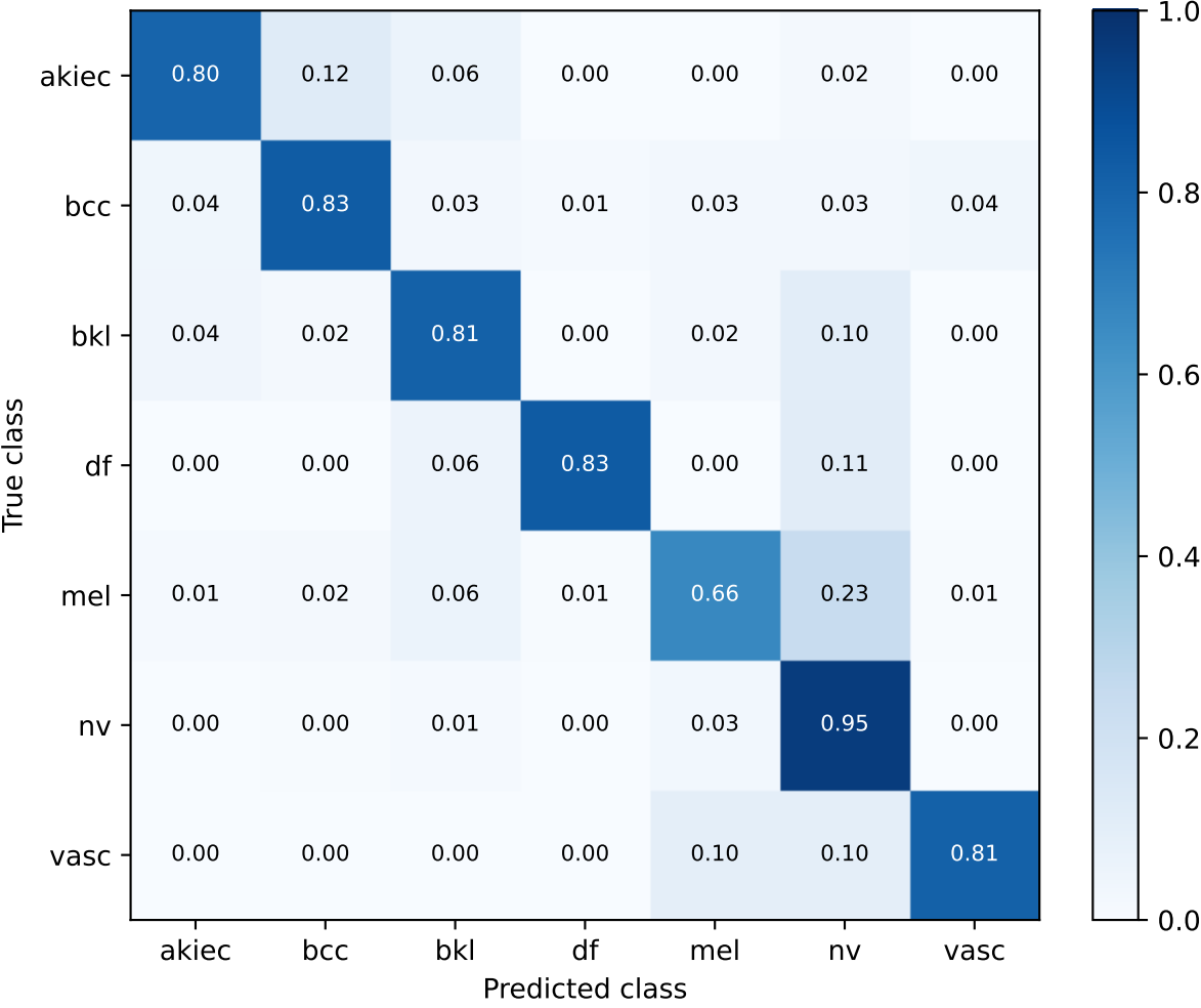
s37_convnext_control_strict_dev_seed42 | post-test strict development Row-normalized confusion matrix
